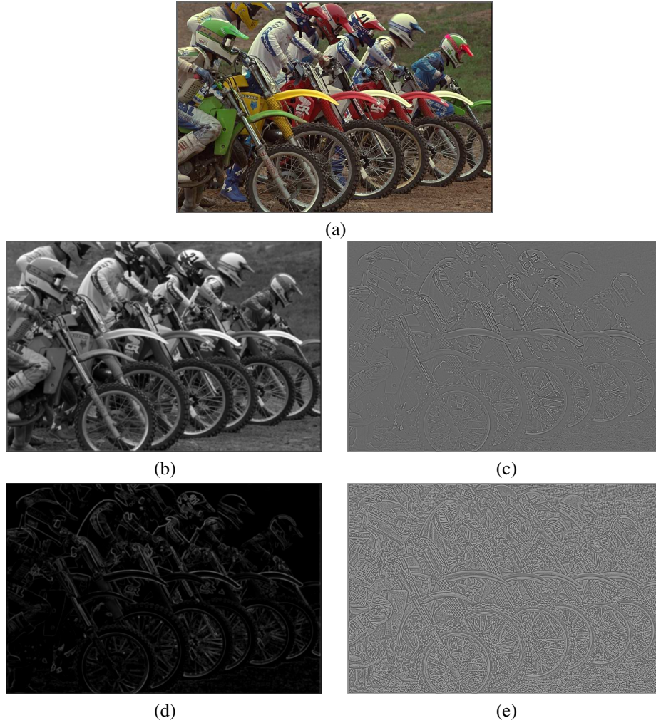
Fig. 3. Effect of the normalization procedure. (a) Original Image I , (b) Local mean field \mu , (c) I - \mu , (d) Local variance field \sigma and (e) MSCN coefficients ((I - \mu)/\sigma)
